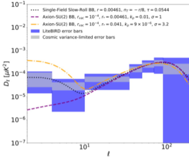
Fig. 2: B-mode power spectra for different inflationary models as compared to cosmic variance (grey bands) and LiteBIRD error bars (blue bands) including foregrounds residuals
