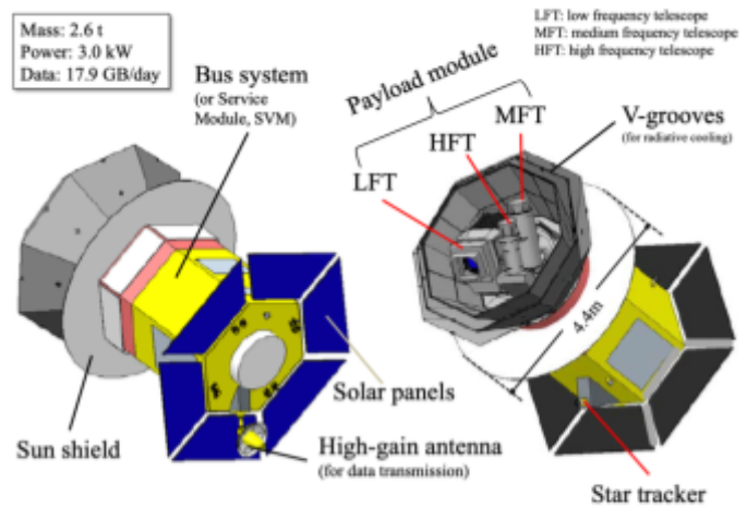
Fig. 6: Conceptual design of the LiteBIRD spacecraft. The payload module houses the Low-Frequency Telescope (LFT), the Mid-Frequency Telescope (MFT) and the High-Frequency Telescope (HFT).
