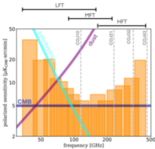
Fig. 4: Frequency bands and their sensitivity in the current LiteBIRD baseline design compared with the main diffuse foregrounds emissions.
