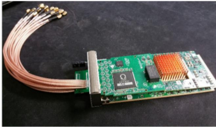
Figure 3.6 Light Readout uTCA digitizer AMC card
