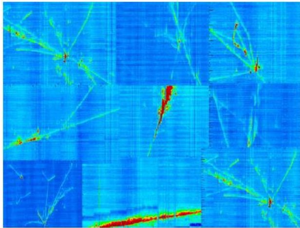
Figure 3.1 A compilation of raw data cosmic ray event displays acquired with the 3x1x1 prototype
