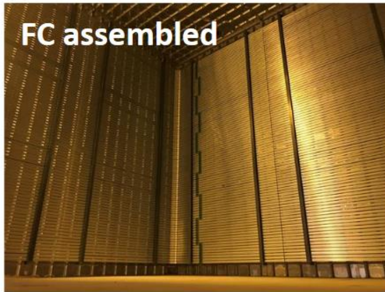
Figure 3.2 Field Cage of ProtoDUNE dual-phase after the completion of its installation inside the cryostat
