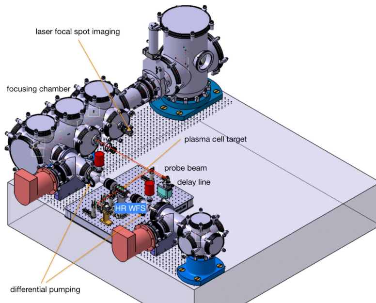
Fig. 6. Plasma cell test bench CAD view with test cell from previous project ESCULAP (K. Wang, N. Delerue et al.) [16]
