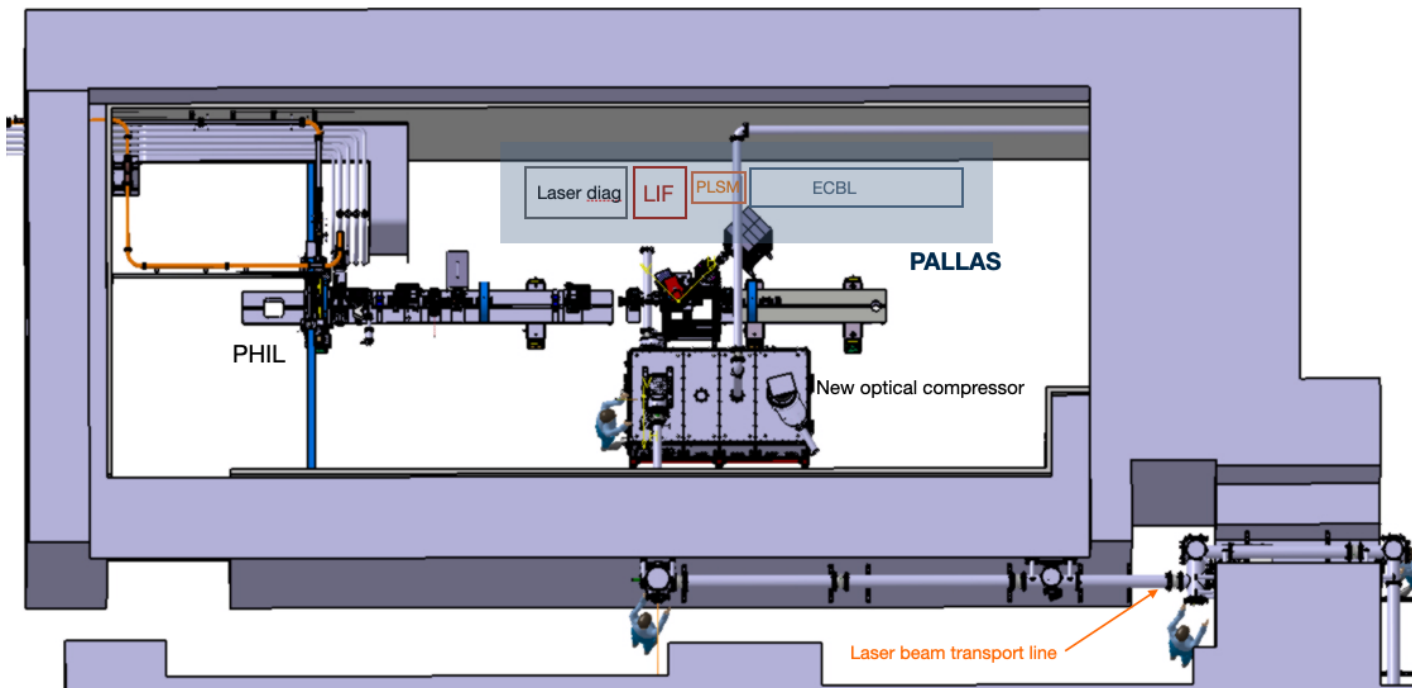
Figure 2 - :top CAD view of the NEPAL experimental hall with the PHIL accelerator and future implementation of the PALLAS LPI beamline with the new optical laser compressor and laser beam transport line
